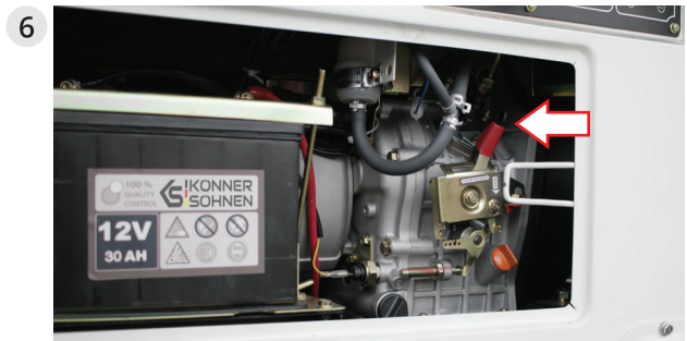
Set the safety switch to "START".
