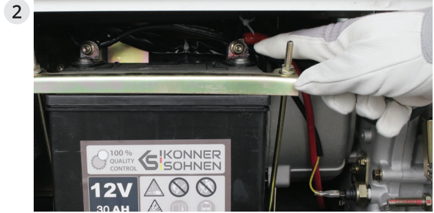
Open the service door. Connect the terminals to the battery: "+" to "+" (red), "-" to "-" (black).
