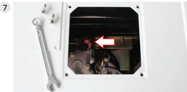
On the top of the generator, unscrew the metal cover behind which the decompressor lever is located. Hold the decompressor lever down.
